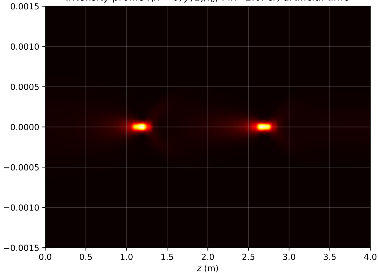
Intensity profile I(x=0, y, z)/I_0 , P_{in}=2.0P_{cr} , artificial time
